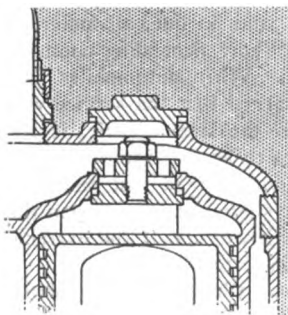
Pierce Cylinder.
